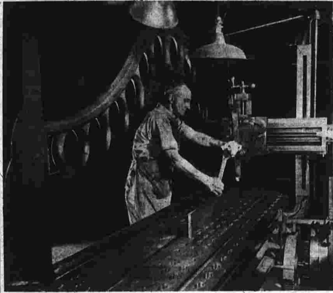
Herold Photo. Ralph Von Deck, 18-Knox St., a machinist at Cheney Bros., makes an adjustment on "The Wreck," a nearly 100 year old open side planer. The curving frame at left rides on supports at other end of the machine and carries the block holding the cutting tool on which Von Deck is working. Because the side at left is open, it allows great clearance for work being machined.
